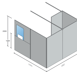
Singular Intermediate Fully Accessible Booth
