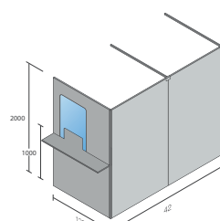
Singular Intermediate Booth
