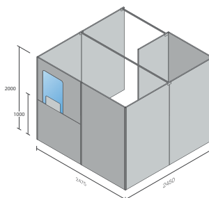
Singular Fully Accessible Master Booth
